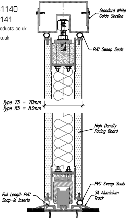
BOTTOM RUNNING
