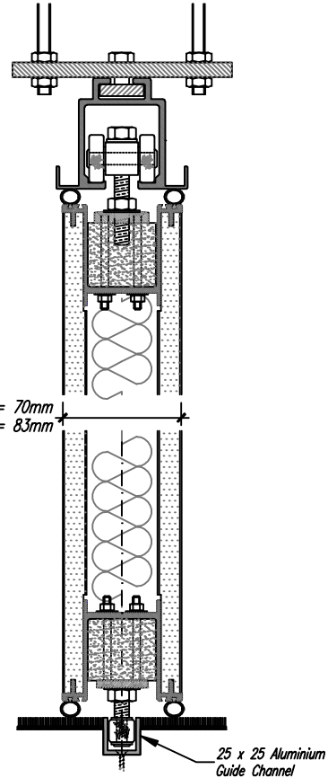
TOP HUNG
